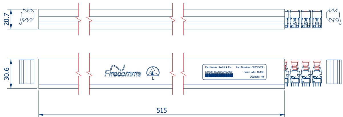
FIGURE 7 Packing tube for Firecomms Vertical RedLink® Receivers
