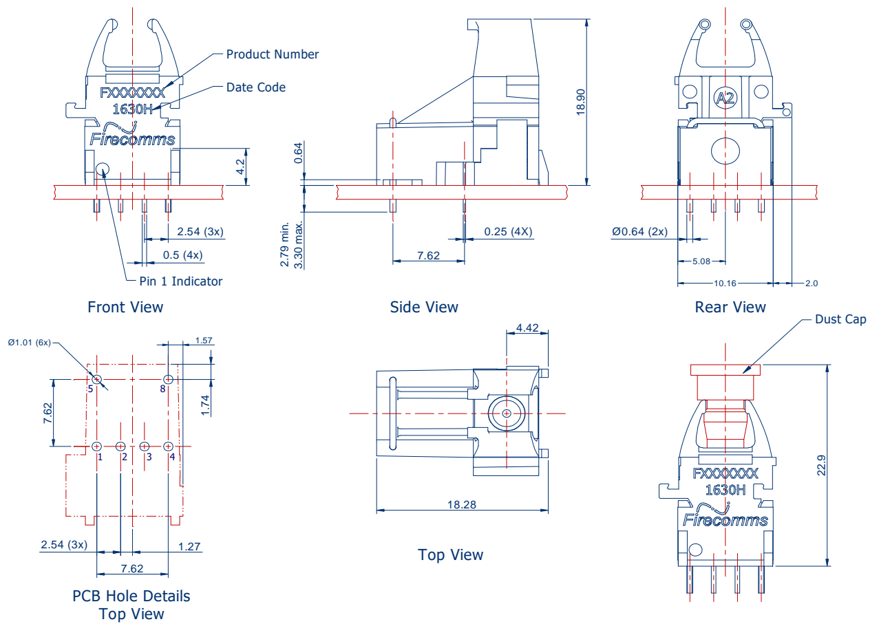
FIGURE 6 Mechanical dimensions of the vertical receivers and PCB footprint, which is a top view. General dimensional tolerance is \pm 0.2 mm
